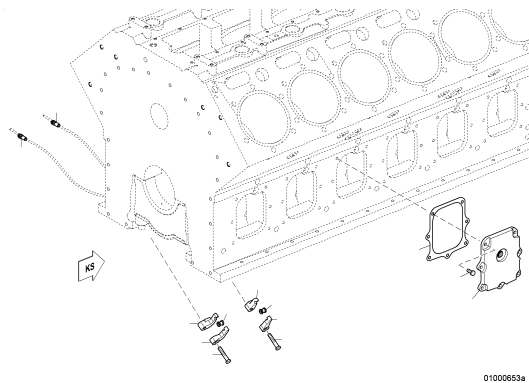
CRANKCASE MONITOR FOR 16V XS595010.00017
