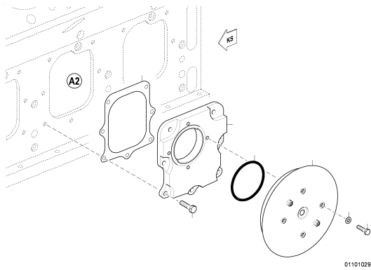
SAFETY VALVE XS594010.00019
